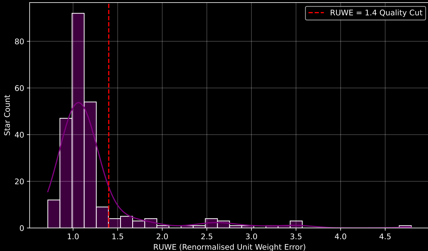
GALAH DR4 Field [7144] RUWE Distribution (n= 248)
