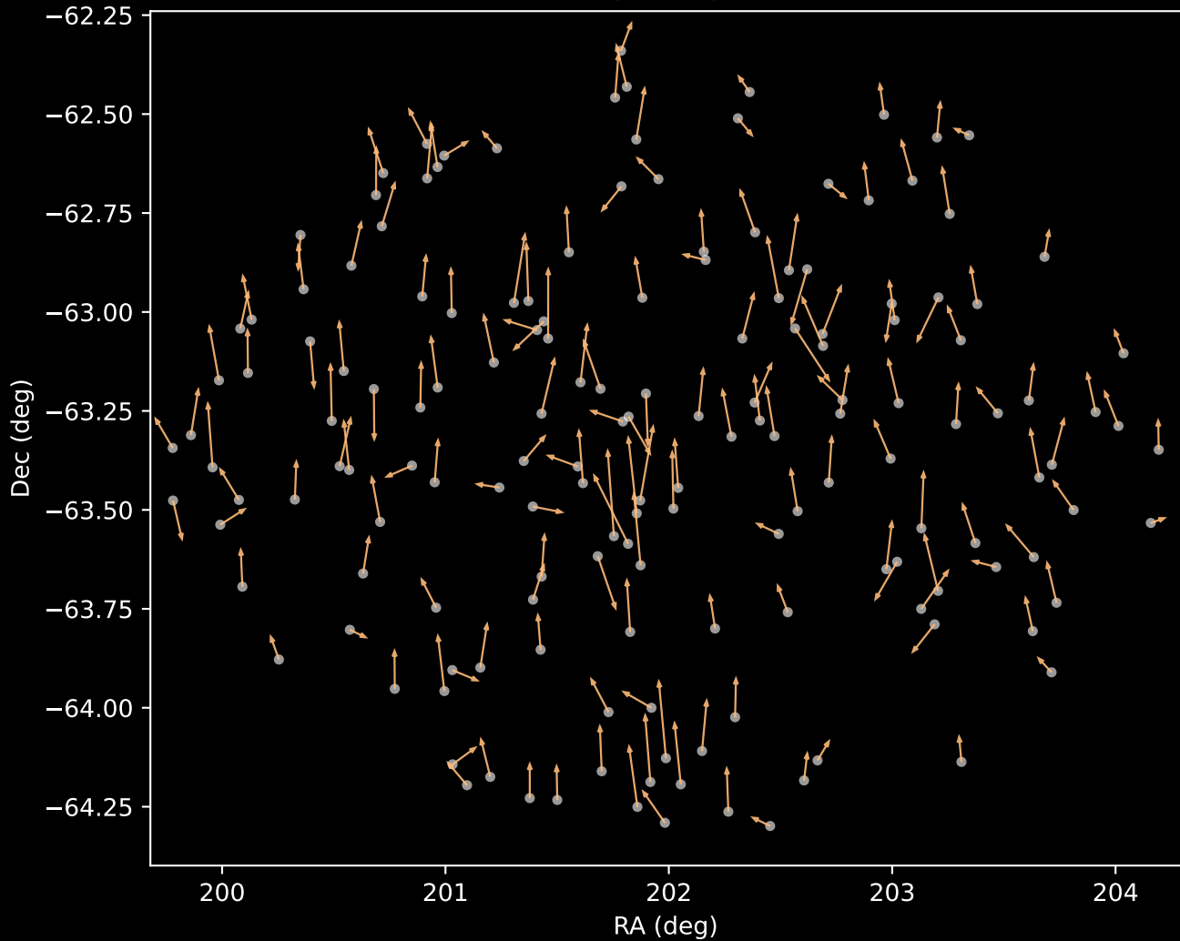
GALAH DR4 Cluster 3 Proper Motion Vectors (n=163)
