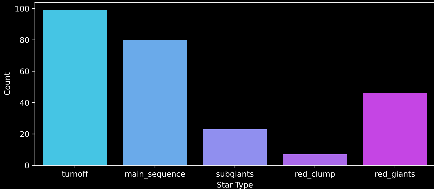
GALAH DR4 Field: [7144] Count plot of Star Type
