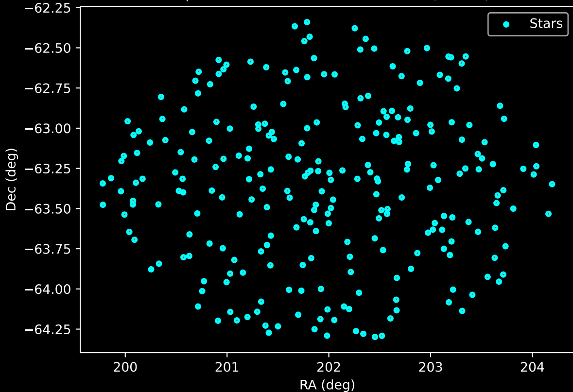
GALAH DR4 Field: [7144] Proper Motion Vectors for Gaia Star Field (n= 255)
